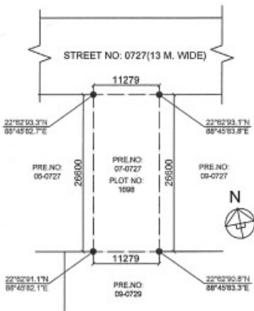
SITE PLAN SCALE 1:450
